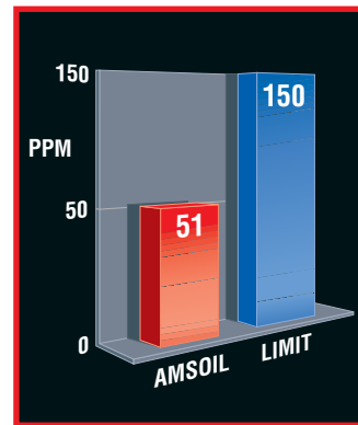
Wear Metal: IRON Even after 409,000 miles, AMSOIL contained only 1/3 the wear metal IRON allowed by Mack condemnation limits.
